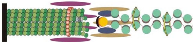
Fig. 2 A schematic representation of the interface between kinetochore microtubule, kinetochore, and centromere DNA. The microtubule (green polymer, left) is nucleated from the spindle pole body (black rod). Chromatin DNA is depicted as a red line wrapped around histone proteins (turquoise). At the centromere (125 bp in budding yeast), there is a unique set of histone proteins Cse4 (Meluh et al. 1998) and scm3 (Camahort et al. 2007; Mizuguchi et al. 2007; Stoler et al. 2007) depicted in yellow. If the DNA adopts an intramolecular loop, the dimension of a loop of nucleosomal chromatin DNA is approximately 2 \times 11.5 \text{ nm} = 23 \text{ nm} . The diameter of the microtubule is 25 nm. The kinetochore is depicted as an array of elongated helices based upon the hydrodynamic properties of the isolated proteins (McAinsh et al. 2003) and determination of molecular protein counts (Joglekar et al. 2006)
