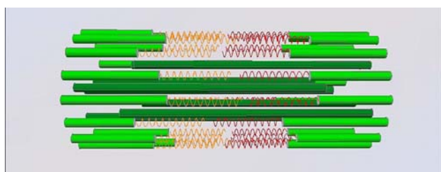
Fig. 1 Proposed view of DNA strands as tension elements in the budding yeast mitotic spindle. Dark green —interpolar microtubules, light green —kinetochore microtubules, orange and red —DNA strands representing intramolecular loops of DNA
